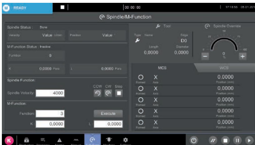
Spindle management
