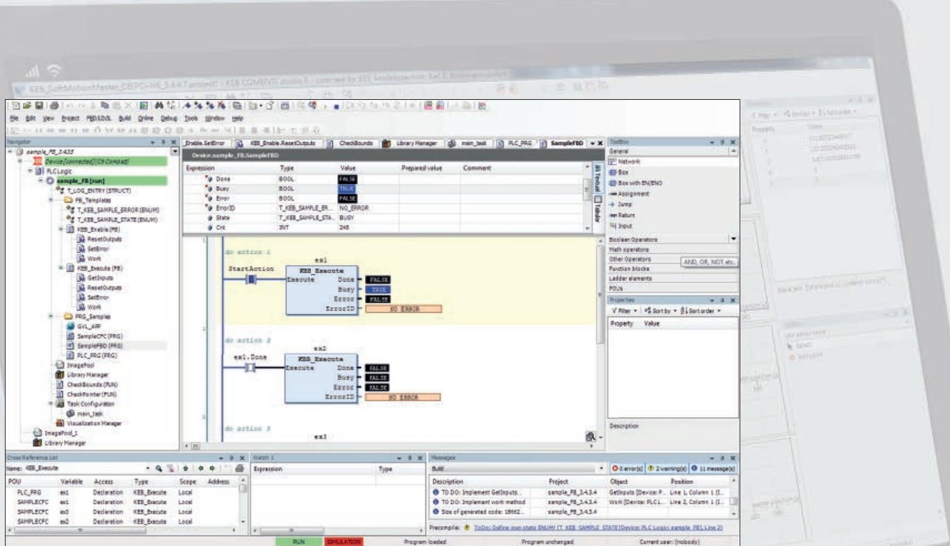
Online depiction
