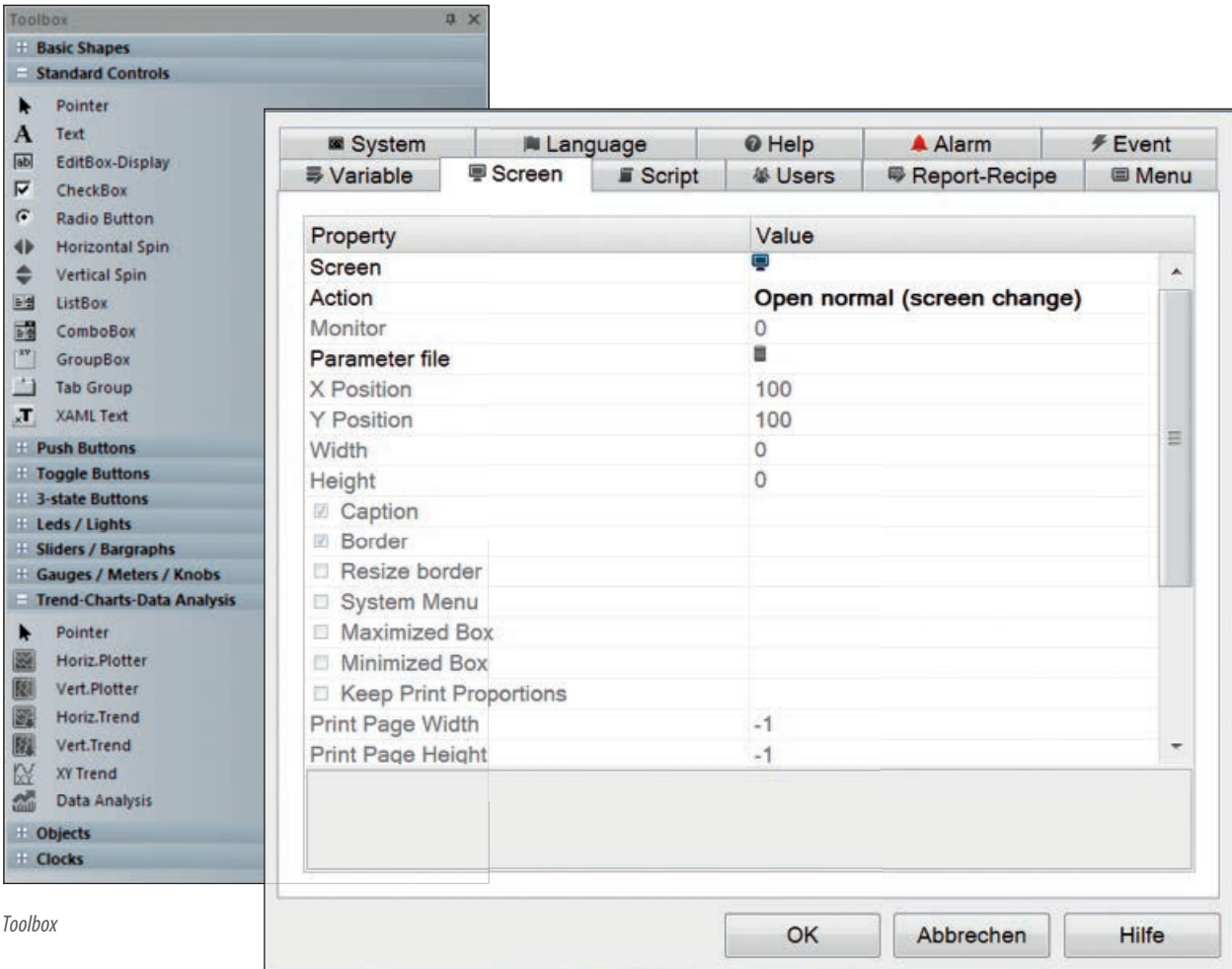
Properties
