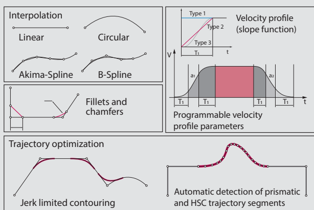
Path generation functions
