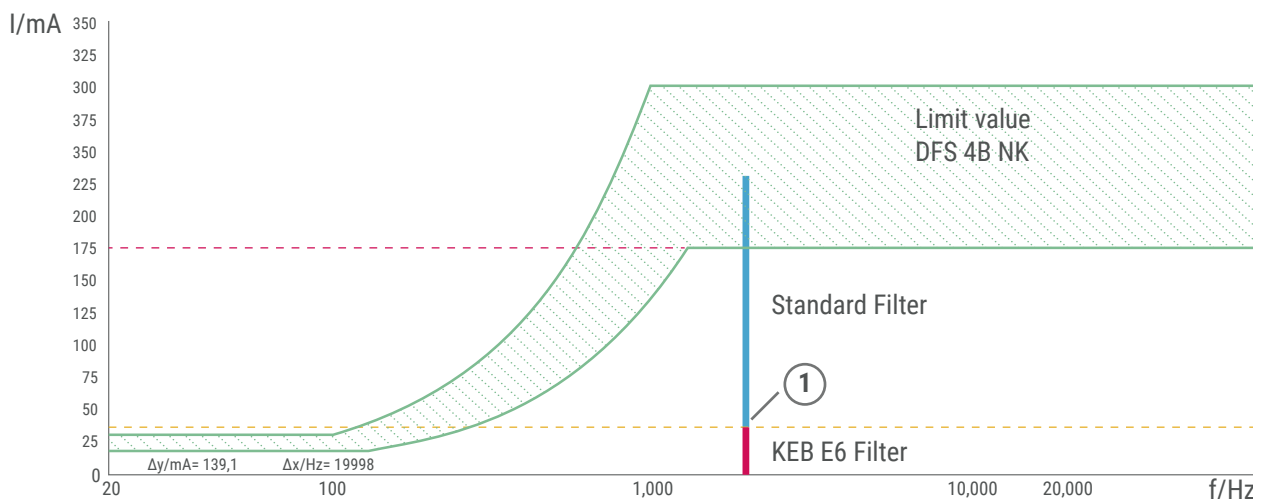
Illustration: Leakage current measurement 22E6T60-1050
